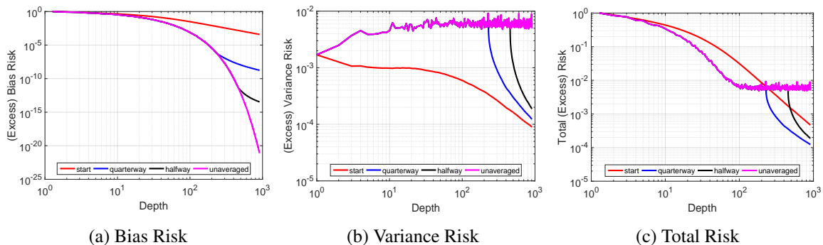
Figure 2: [Zoom in to see detail] Effect of tail-averaging with mini-batch size of b_{thresh} = 11 .
