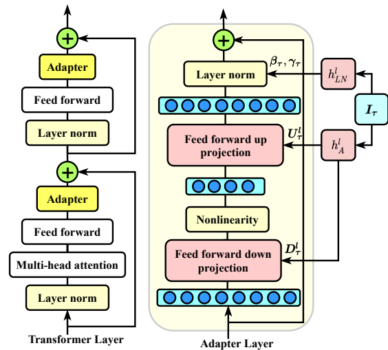
Figure 1: Left: Adapter integration in the T5 model. Right: Our HYPERFORMER adapter architecture. Following Houshy et al. (2019), we include adapter modules after the two feed-forward layers. The Adapter hypernetwork h_A^l produces the weights ( U_\tau^l and D_\tau^l ) for task-specific adapter modules conditioned on an input task embedding I_\tau . Similarly, the layer normalization hypernetwork h_{LN}^l generates the conditional layer normalization parameters ( \beta_\tau and \gamma_\tau ). During training, we only update layer normalizations in T5, hypernetworks, and task embeddings. The compact HYPERFORMER++ shares the same hypernetworks across all layers and tasks and computes the task embedding based on task, layer id, and position of the adapter module (§2.4).
