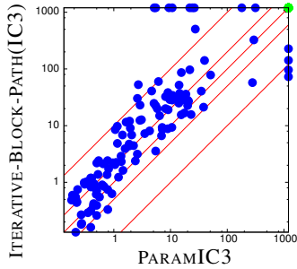
Fig. 2. Comparison between PARAMIC3 and ITERATIVE-BLOCK-PATH(IC3).
