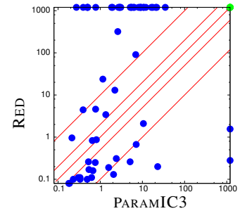
Fig. 4. Comparison between PARAMIC3 and RED.
