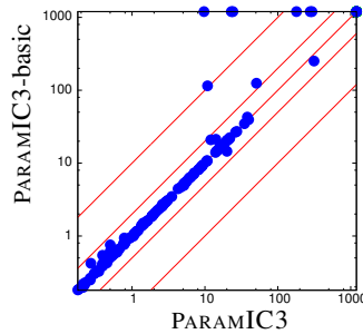
Fig. 3. Comparison between PARAMIC3 and PARAMIC3-basic.
