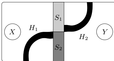
Figure 3: Separators in the proof of Lemma 3.4.
