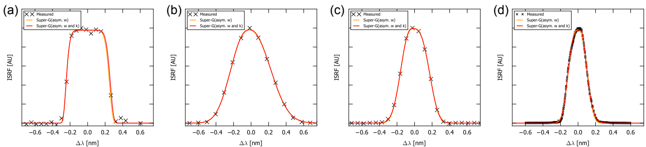
Figure A3. Exemplary TROPOMI ISRF for the UV (a), UVIS (b), NIR (c), and SWIR (d) at the detector edges. Crosses indicate the pre-launch measurements (provided by Antje Ludewig (UV, UVIS, NIR) and Paul Tol (SWIR), personal communication, 2016). Lines show the best matching parameterizations S_{a_w} and S_{\text{asym}} . The respective fit parameters are listed in Table A1.
