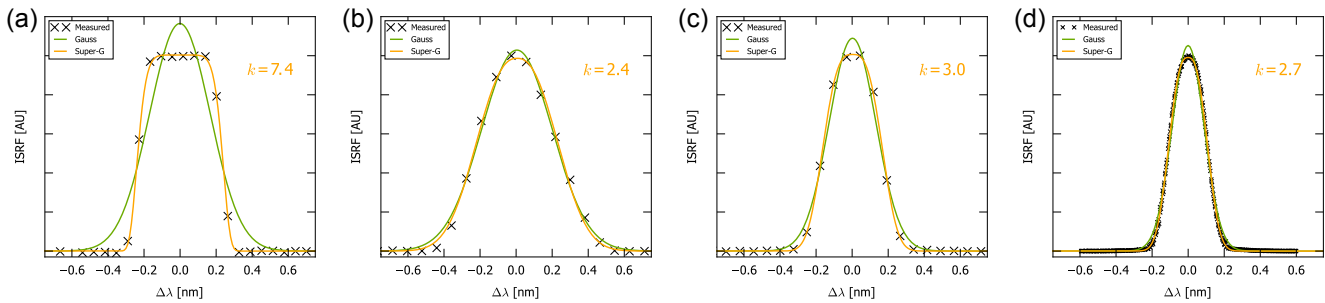
Figure 6. Exemplary TROPOMI ISRF for the UV (a), UVIS (b), NIR (c), and SWIR (d) at the detector centers. Crosses indicate the pre-launch measurements (provided by Antje Ludewig (UV, UVIS, NIR) and Paul Tol (SWIR), personal communication, 2016). Lines show the best matching parameterizations G and S . The respective fit parameters are listed in Table 5.
