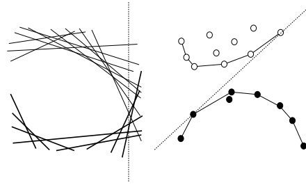
Figure 2. First non-positive swap: (a) in line arrangement, right-most point above lines from tree edges and below lines from non-tree edges; (b) in dual point arrangement, line with highest slope above points from tree edges and below points from non-tree edges.
