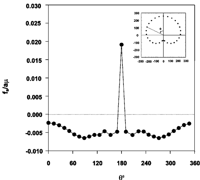
FIG. 5. Angular variation of the self force (units of \sigma/aua ) in copper for the Frank-Read source after segment annihilation. The angle \theta is defined in the insert. All distances on the figure are in units of the lattice constant.
