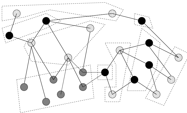
Figure 1: An example of a graph in \mathcal{G}_n .
