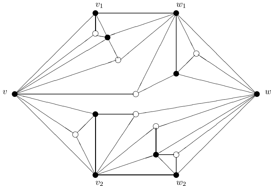
Figure 4: Illustration of a possible worst-case scenario for Case 1 . Empty circles represent white vertices, and filled circles black vertices.
