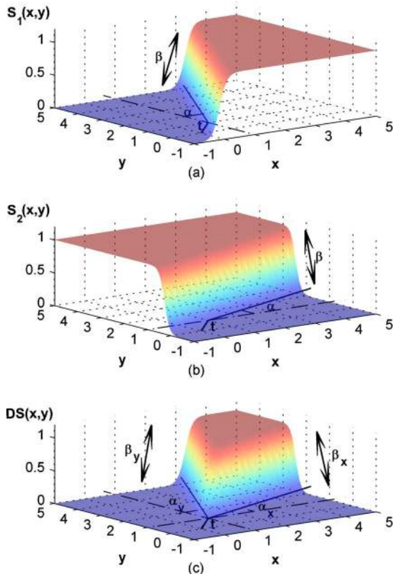
Fig. 4. (Color online) Two-dimensional sigmoid functions. (a) S_1 , sigmoid function oriented in the x-axis direction (b) S_2 , sigmoid function oriented in the y-axis direction (c) DS, product of two differently oriented sigmoid functions generates a plateau with some of the properties needed for the membership function.
