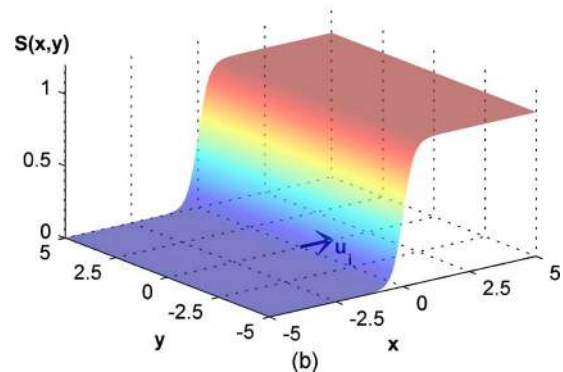
Fig. 3. (Color online) (a) Sigmoid function in one dimension. The value of \beta determines the slope of the function. (b) Sigmoid function in two dimensions. Vector \mathbf{u}_1 determines the axis in which the function is oriented.
