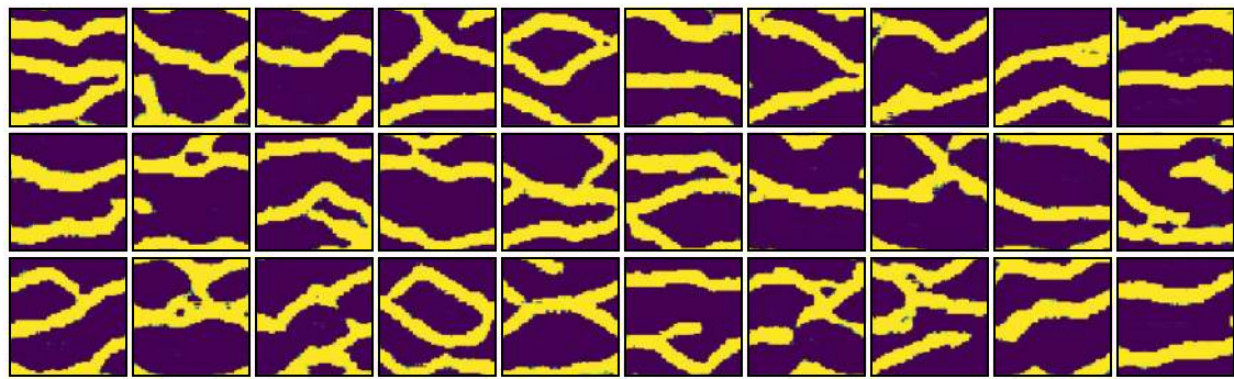
(a) G(z)
