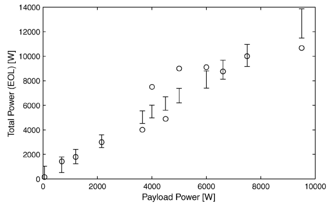
Fig. 3 P_{eol} estimates using Eq. (9) with 95% confidence intervals.
