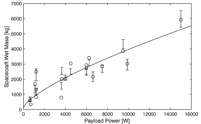
Fig. 2 Wet mass estimates using Eq. (6) with 95% confidence intervals superimposed over the FCC data; —, follows Eq. (5).
