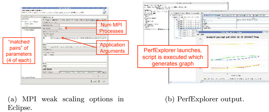
Fig. 4. The results of running the MPI weak scaling study - PerfExplorer is executed, and the results of the study are visualized in one chart.
