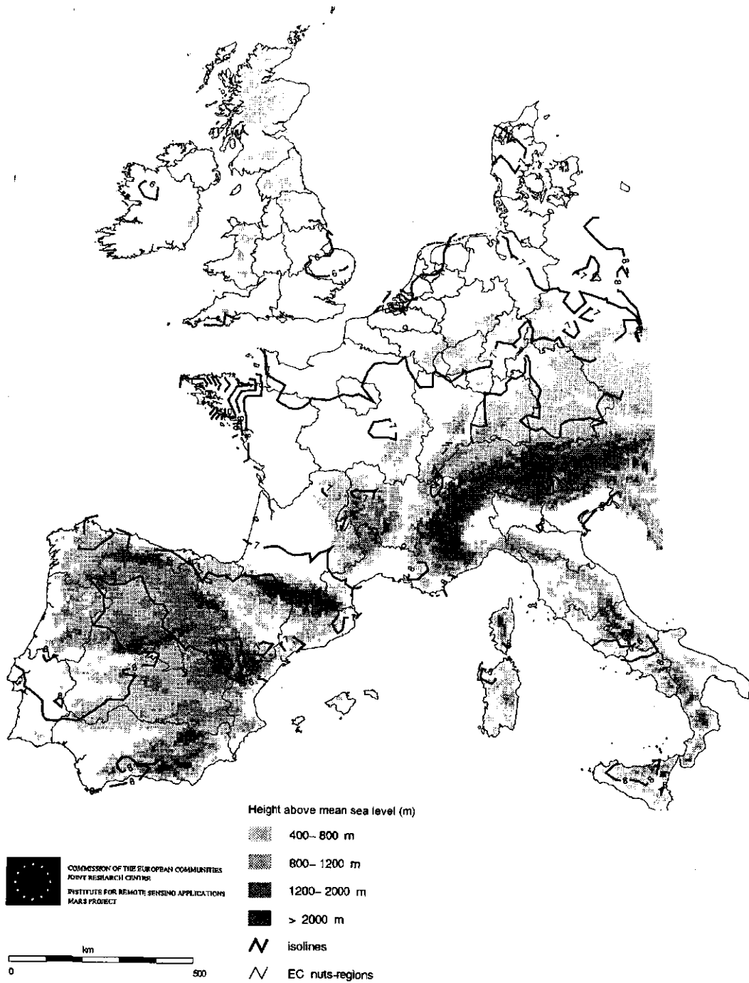
Fig. 20 Amplitude of radiation - wet conditions [MJ m -2 d -1 ]
