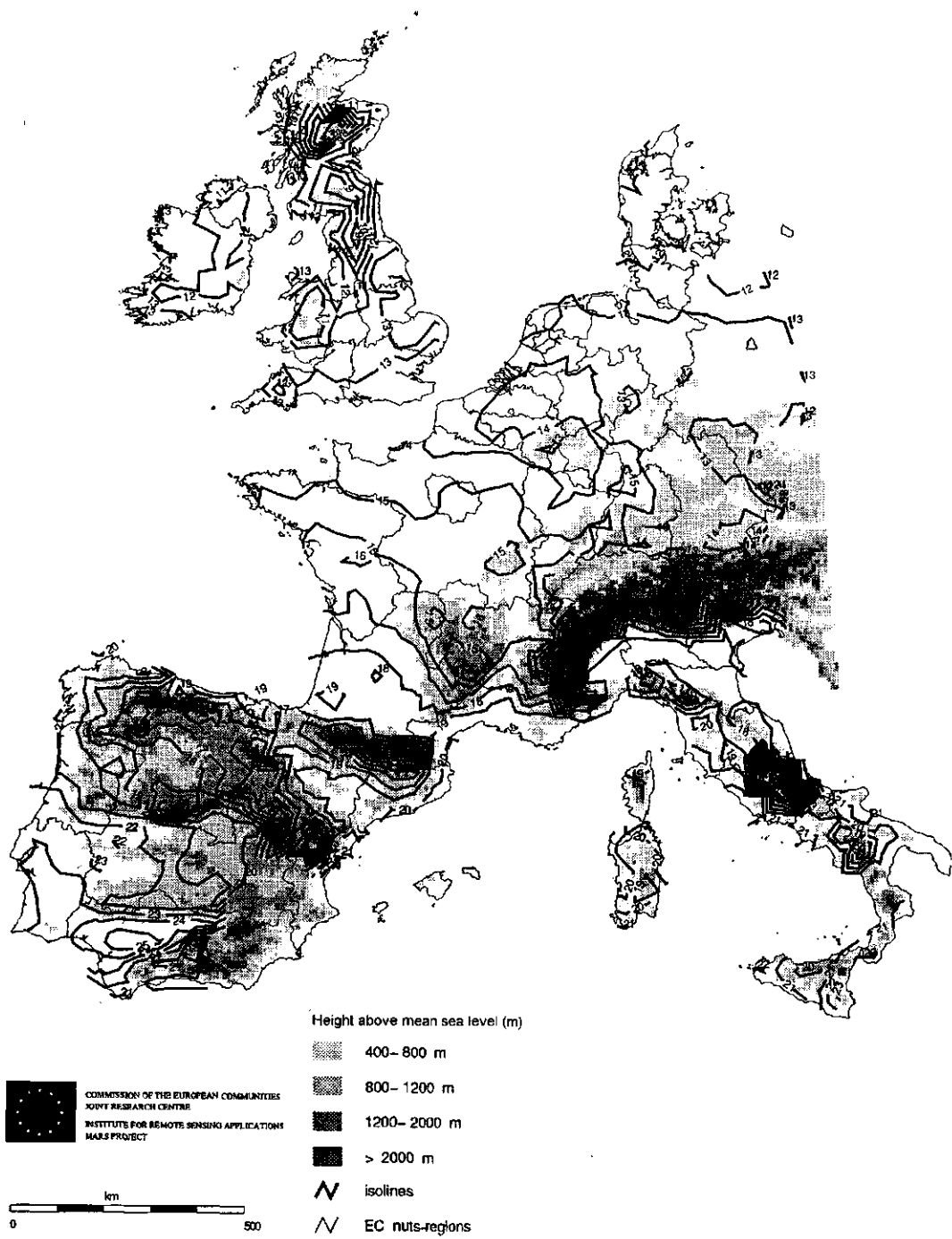
Fig. 11 Yearly average of maximum temperature - dry conditions [ ^{\circ} C]
