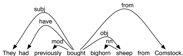
Figure 2.4: Lin and Pantel (2001) extracted paraphrases which had similar syntactic contexts using dependency parses like this one
