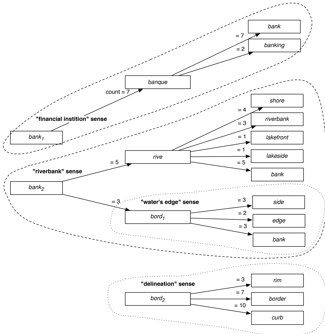
Figure 3.11: If we treat words with different senses as different items then their alignments are partitioned. This allows us to more draw more appropriate paraphrases, if we are given the word sense of the original phrase.
