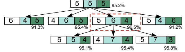
Figure 4: An example of how Paraprox’s bit tuning finds the number of bits assigned to each input for the BlackScholesBody function. The lookup table has 32768 entries and its address is 15 bits wide. The output quality is printed beside each node. Bit tuning’s final selection is outlined with a dotted box.
