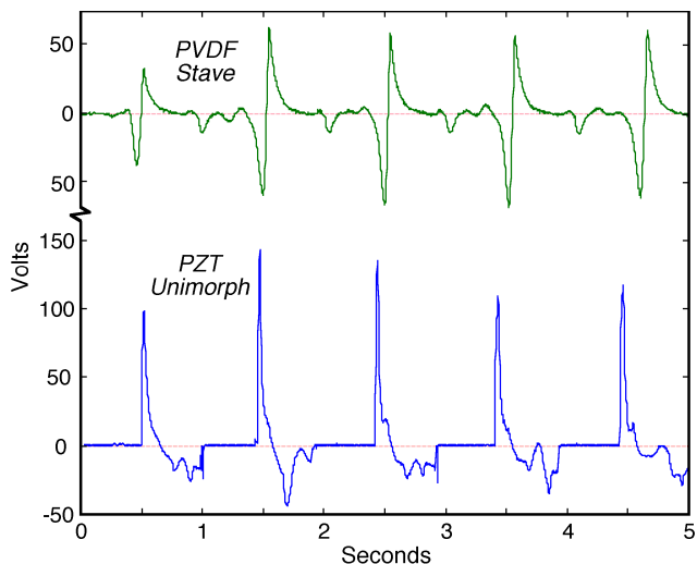
Figure 8: Voltage into 250K load from piezo generators
