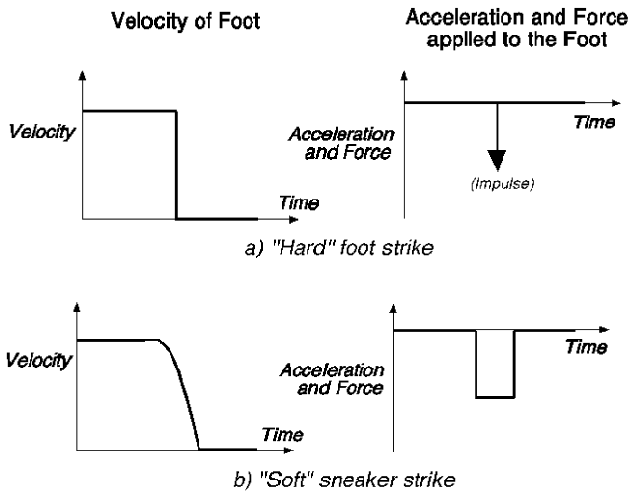
Figure 1: Dynamics for hard vs. cushioned foot strikes
