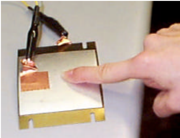
Figure 5: A Thunder PZT unimorph under test
