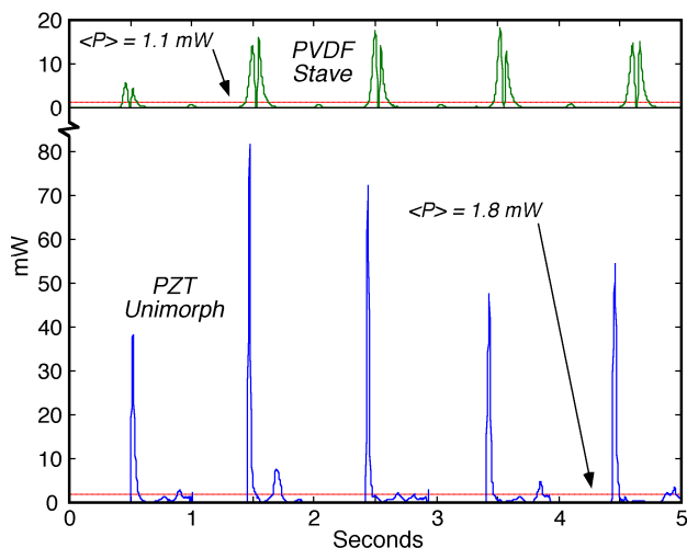
Figure 9: Resulting power output from piezo generators
