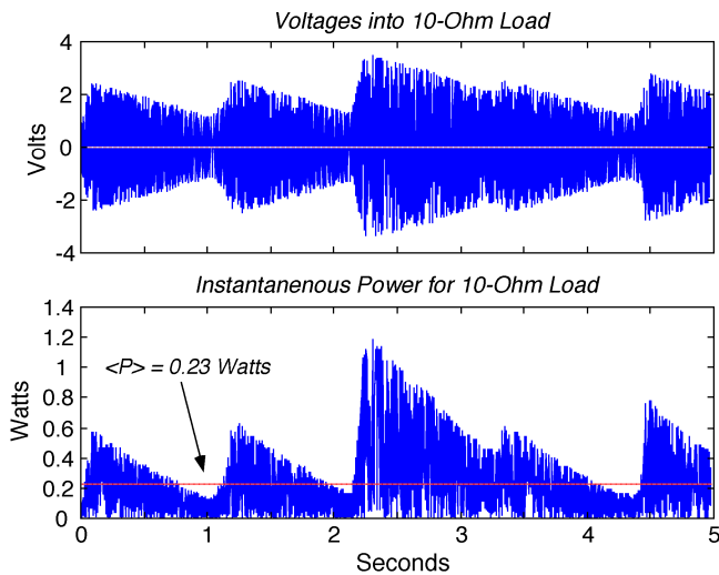
Figure 10: Performance of magnetic generator
