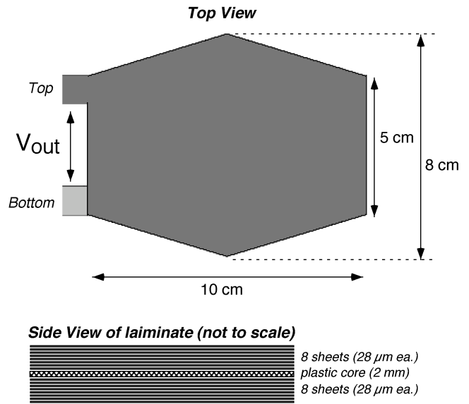
Figure 3: Layout of the PVDF Power Insole
