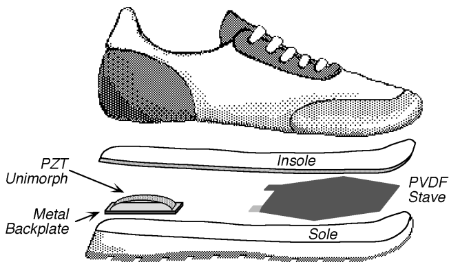
Figure 7: Exploded view showing integration of piezos
