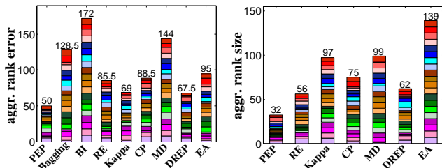
Figure 1: The aggregated rank on the test error and on the size for each method (the smaller the better).
