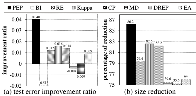
Figure 3: Average performance improvement and size reduction from the Bagging of 100 base classifiers for the MHAR task (the larger the better).
