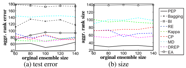
Figure 2: The aggregated rank of each method pruning the Bagging of \{60, \dots, 140\} classifiers (the smaller the better).
