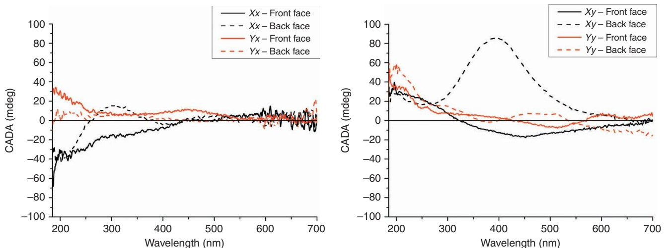
Figure 3 Comparison of spectral circular polarization degree of attenuation (CADA) for four configurations of writing and polarization direction from the two faces of the samples ( Xy , Yy , Xx and Yx ). Laser writing conditions: wavelength: 1030 nm, pulse duration: 300 fs, repetition rate: 500 kHz, numerical aperture (NA): 0.6, energy: 1\ \mu\text{J} per pulse, writing speed: 500\ \mu\text{m s}^{-1} , focal depth: 192\ \mu\text{m} .
