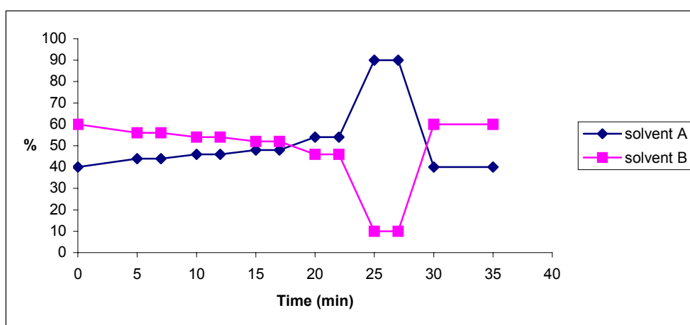
Figure 5. HPLC-FLD gradient used for the elution of OTA and metabolites
