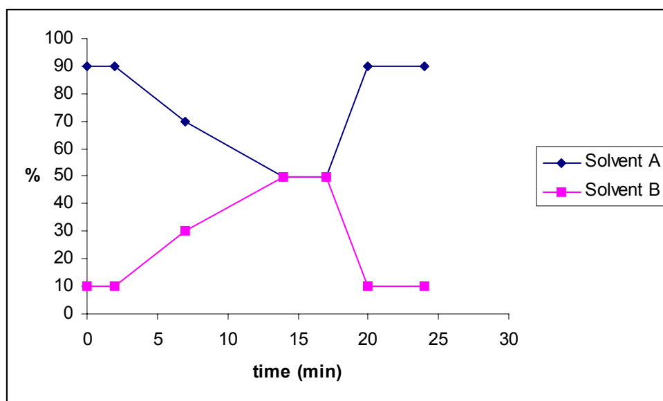
Figure 6. LC-MS/MS gradient used for the elution of ochratoxin A and its metabolites.
