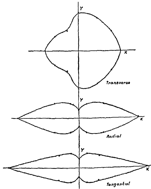
FIG No 4 Young's Modulus of [unclear]
