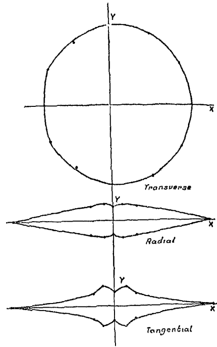
FIG No 2 Young's Modulus of Terminalia Paniculata ELASTIC PROPERTIES OF WOOD
