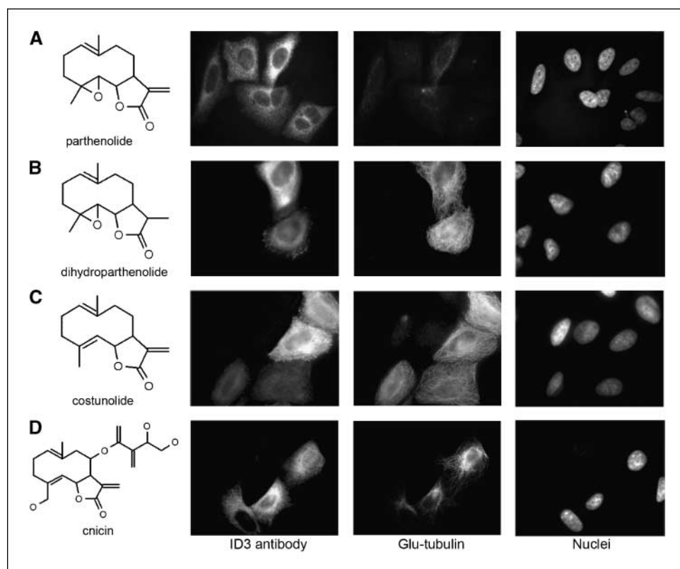
Figure 5. Comparison of the effect of several structural analogues of V18 and V19 on TCP activity evaluated after ID3 microinjection. HeLa cells were microinjected with the TTL inhibitory antibody ID3 and incubated for 4 h with the different compounds as indicated. They were then fixed and processed for immunofluorescence as described in Materials and Methods. Cells were triple stained using an antimouse Cy3-conjugated antibody to mark ID3 microinjected cells, L4 antibody and Alexa Fluor 488-conjugated secondary antibody to visualize Glu-tubulin, and Hoechst 33258 to visualize nuclei as indicated.
