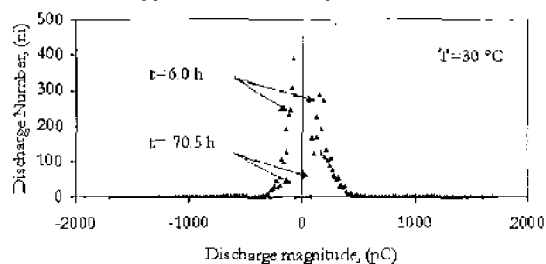
Figure 8. Discharge amplitude distributions detected under a life test at 30 kV and 30°C.
