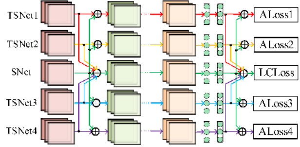
Figure 3. The architecture of PS-MCNN-LC, which shares the architecture of PS-MCNN but is different at the loss function.
