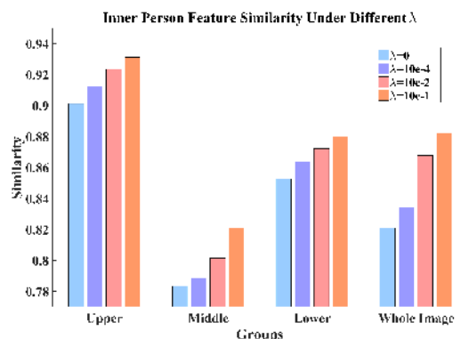
Figure 4. Inner person feature similarity under different \lambda of four groups. The larger the \lambda , the more similar the features of the same identity.
