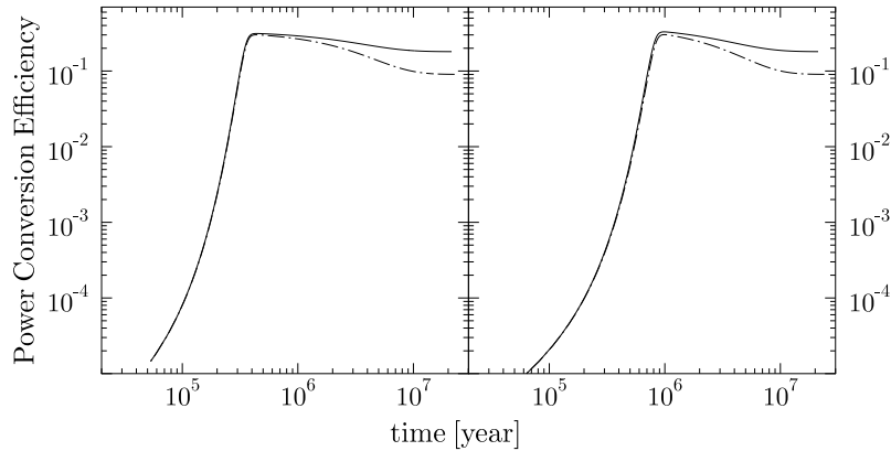
Figure 1. The temporal evolution of the power conversion efficiency to the nonthermal nuclei for two SB scale sizes R = 220 pc (solid lines) and R = 100 pc (dot-dashed lines). Both nonrelativistic (left panel) and relativistic (right panel) particle injection regimes are shown.
