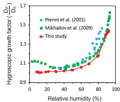
Figure 2. Measured hygroscopic growth factor (HGF) of oxalic acid particles at different RH conditions. D_p is the particle diameter at an elevated RH, and D_0 (100 nm) is the initial diameter of oxalic acid particles at \text{RH} = 8\% .
