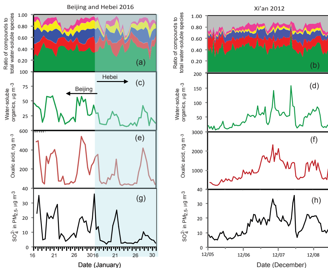
Figure 3. Measurements of water-soluble organic matter (WSOM) of \text{PM}_{2.5} collected in Beijing and Hebei Province during the winter of 2016 (a, c, e, g) and in Xi'an during the winter of 2012 (b, d, f, h). In panels (a) and (b), the green, red, blue, yellow, pink, and gray colors represent WSOM, sulfate, nitrate, ammonium, chloride, and the others (i.e., the sum of \text{Na}^+ + \text{Ca}^{2+} + \text{Mg}^{2+} + \text{K}^+ ), respectively.
