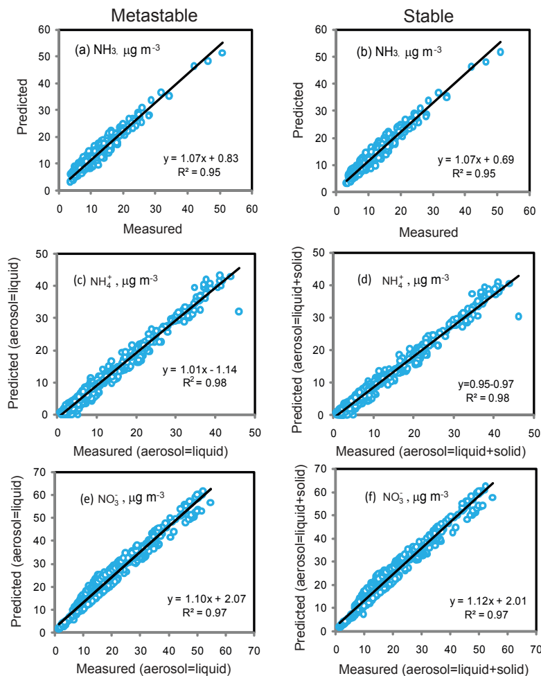
Figure 4. Comparison of measured \text{NH}_3 , \text{NH}_4^+ , and \text{NO}_3^- concentrations with those predicted by ISORROPIA-II model using the forward mode under the metastable (a, c, e) and stable assumptions (b, d, f).
