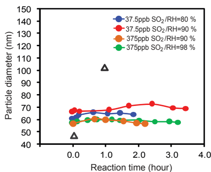
Figure 1. Size evolution of ammonium sulfate (circle dots) and oxalic acid (black triangles) particles after exposure to \text{SO}_2 , \text{NO}_2 , and \text{NH}_3 at different RH levels. Variations in mobility diameter ( D_p ) of the particles as a function of reaction time. The symbols with different colors denote measurements with exposure to different \text{SO}_2 , \text{NO}_2 , and \text{NH}_3 concentrations and RH levels. For the ammonium sulfate particles exposure experiment, two levels of \text{SO}_2 were used, which are 37.5 and 375 ppb, respectively, while the \text{NO}_2 concentration is 375 ppb, and the \text{NH}_3 concentration is 500 ppb. For the oxalic acid particles exposure experiment, the \text{SO}_2 concentration is 250 ppb, the \text{NO}_2 concentration is 250 ppb, and the \text{NH}_3 concentration is 1 ppm (The data of oxalic acid growth are cited from the previous study by Wang et al., 2016).
