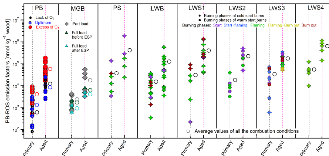
Figure 1. PB-ROS emission factors ( EF_{\text{ROS}} ) for all tested combustion devices under different operating and aging conditions. Open circles represent the average values of all the experimental data points for each condition. PB denotes pellet boiler; MGB, moving grate boiler; PS, pellet stove; LWB, log wood boiler; LWS n , log wood stove n ( n = 1, 2, 3, 4 ). Each data point represents one experiment. For each device, primary EF_{\text{ROS}} appear on the left side (gray dashed line) and aged EF_{\text{ROS}} on the right side (pink dashed line).
