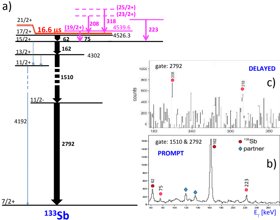
Fig. 3. (a) Partial level scheme of ^{133}\text{Sb} , showing (in black) the known level scheme below the long lived 21/2^+ isomer [20, 21]. New transitions are given as gray/pink, thick arrows originating from states with tentative spin assignments. They were observed by studying either \gamma coincidences between prompt transitions, as shown in panel (b) or between delayed and prompt ones, as shown in panel (c). Both spectra were taken from the fission data on the ^{235}\text{U} target (see the text for details).
