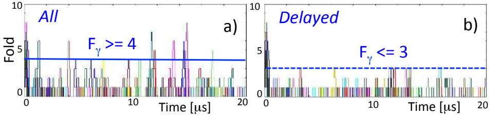
Fig. 1. (a) Ge fold distributions for 10 sequences of events in a 20 \mu s time window, after a prompt fission event (see the text for details). It is seen that in this time range \approx 50\% probability exists for a new prompt fission event (with fold F_\gamma \geq 4 ). (b) Ge fold distributions for 10 events in a 20 \mu s time window, after a prompt fission event, which satisfy the condition F_\gamma \leq 3 for delayed transitions in the interval 200 ns up to 20 \mu s. This allows to reject more than 85% fission events in the delayed time window.
