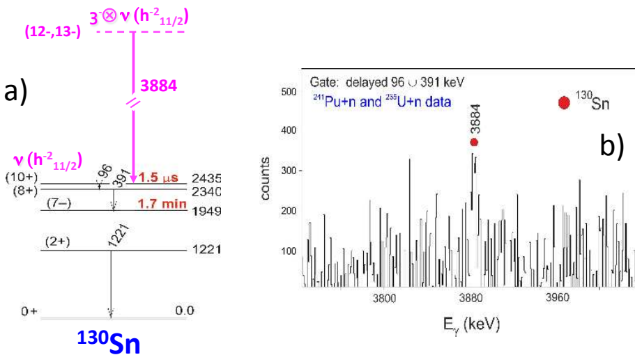
Fig. 4. (a) Partial level scheme of ^{130}\text{Sn} , showing (in black) the known decay below the long lived 10^+ isomer [17]. Panel (b) shows the spectrum of prompt transitions observed in coincidence with the 96 and 391 keV lines depopulating the isomer. The newly found 3884 keV line, feeding the isomer, is suggested to decay from a state arising by coupling the two-neutron-hole state \nu(h_{11/2}^{-2})10^+ to the 3^- phonon of the ^{132}\text{Sn} core, similarly to what found in the case of ^{206}\text{Pb} [4] (see the text for details).
