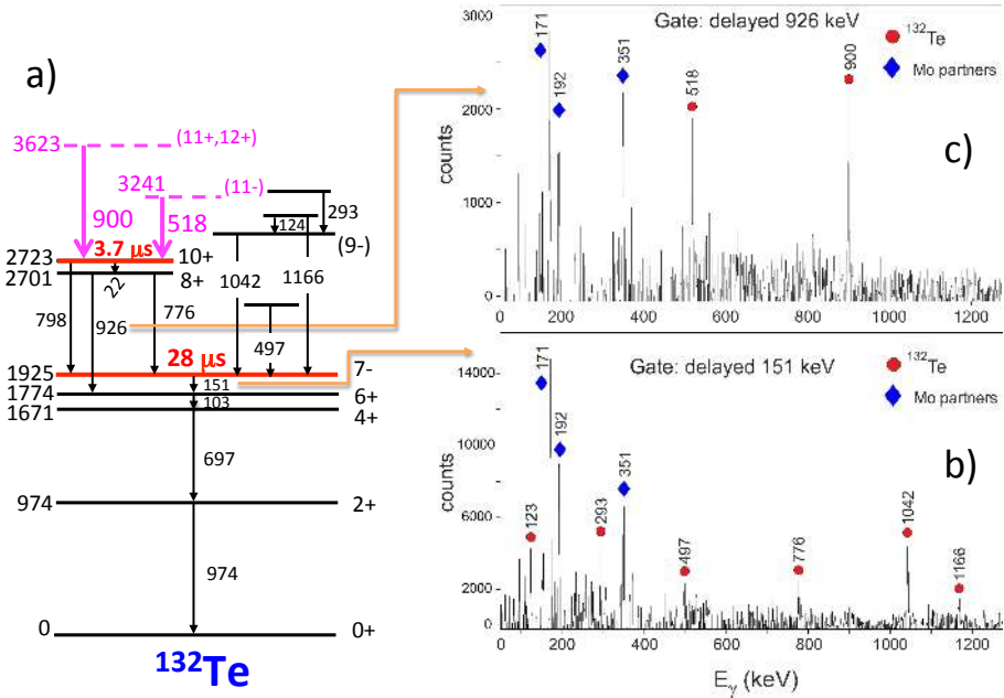
Fig. 2. (a) Partial level scheme of ^{132}\text{Te} showing, in black, the known level scheme below the long lived 7^- and 10^+ isomers and states observed in \beta -decay studies [18, 19]. New transitions found in this work are given as gray/pink, thick arrows originating from states with tentative spin assignments. They were observed by studying \gamma coincidences between delayed and prompt transitions, as shown in panels (b) and (c) in the case of gates set on the 151 and 962 keV lines, respectively (see the text for details).
