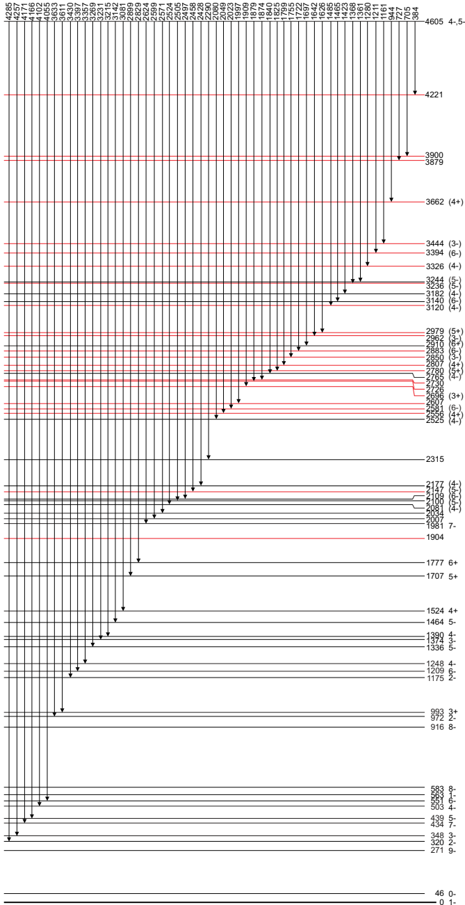
Fig. 5. Partial level schemes of ^{210}\text{Bi} obtained by cold-neutron capture, showing primary decay transitions only. Newly found states are marked in gray/red [23].
