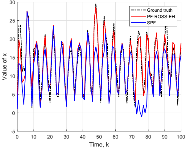
Fig. 2: Estimation results of PF-ROSS-EH and SPF.
