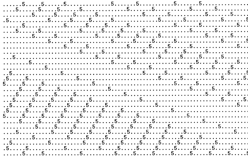
FIG. 3. Space-time plot for CA-184/5 and subcritical density.
