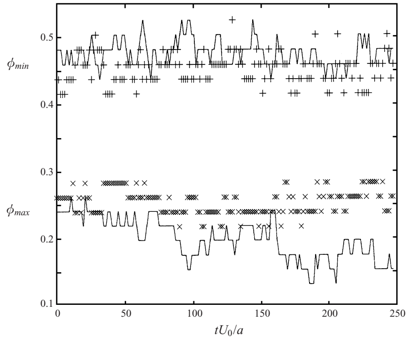
FIGURE 16. \phi_{min} and \phi_{max} as a function of time for a simulation with N = 1024 and \phi = 0.35 . The solid lines represent sedimenting suspensions with St = 100 and the pluses and the crosses represent a hard-sphere system with the same value of T_{\parallel} .
