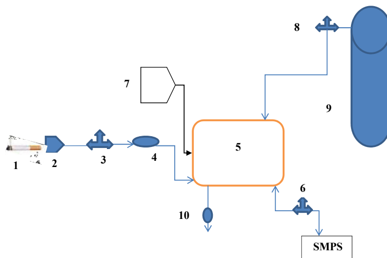
Fig. 1. Mainstream cigarette smoke analysis setup 1) cigarette 2) cigarette holder 3) MCS mass flow controller 4) suction pump (1–3 L/min) 5) dilution chamber 6) flow controller for scanning mobility particle sizer (SMPS) 7) Mouth piece for collection of exhaled cigarette smoke 8) N 2 nitrogen cylinder flow controller 9) N 2 cylinder for dilution 10) pump for dilution chamber evacuation.
