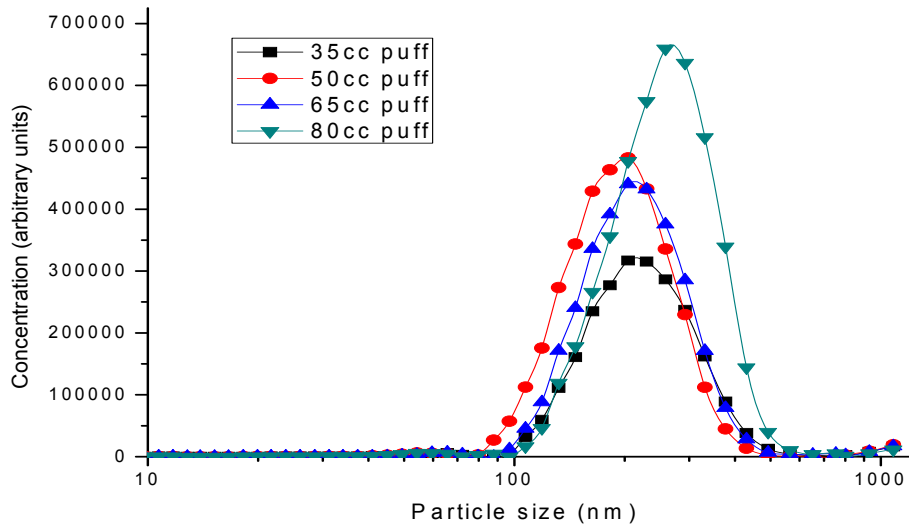
Fig. 4. Particle size distribution for various puff volumes (35 mL, 50 mL, 65 mL and 80 mL).
