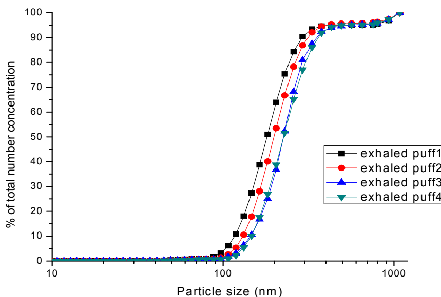
Fig. 7. Cumulative distribution plot of exhaled cigarette smoke for initial four puffs.
