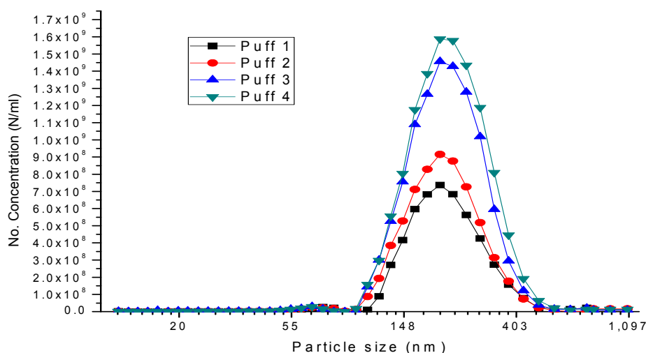
Fig. 2. Mainstream cigarette smoke particle size distribution for initial four puffs, puff duration 2–3 second at flow rate of 1.1 \pm 0.01 L/min.
