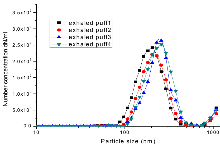
Fig. 6. Particle size distribution of puff wise exhaled cigarette smoke measured with SMPS.
