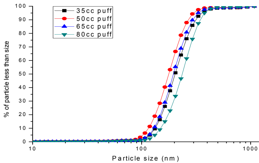
Fig. 5. Cumulative number size distribution of mainstream cigarette smoke for different puff volume (35 mL, 50 mL, 65 mL and 80 mL).
