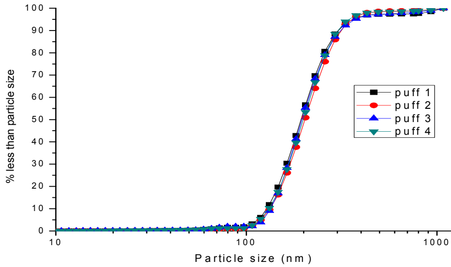
Fig. 3. Mainstream cigarette smoke cumulative size distribution on log probability graph for initial four puffs.
