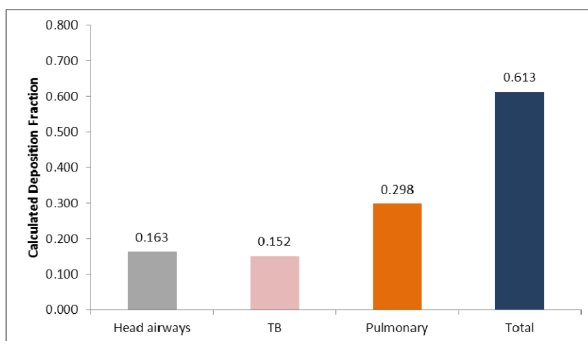
Fig. 9. Calculated deposition fraction for Mainstream cigarette smoke in Entire lung using MPPD model.
