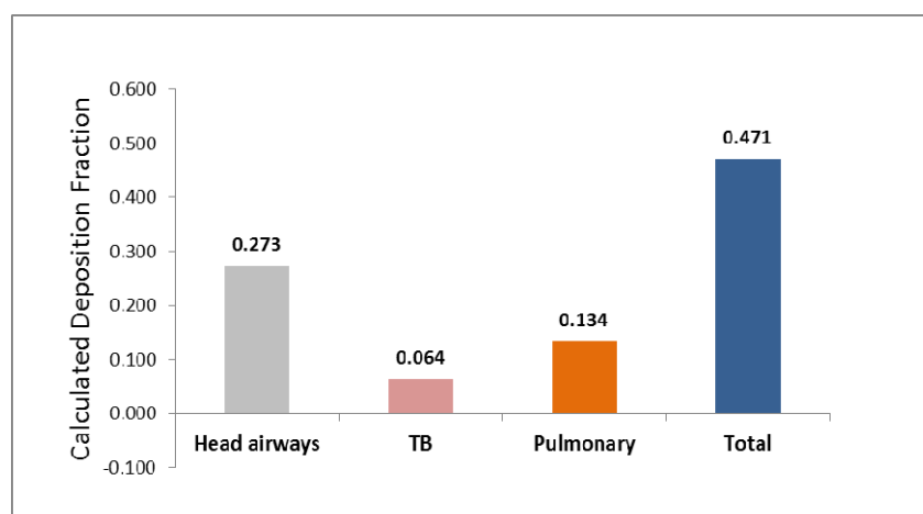
Fig. 10. Deposition fraction for exhaled cigarette smoke for entire lung using MPPD model.
