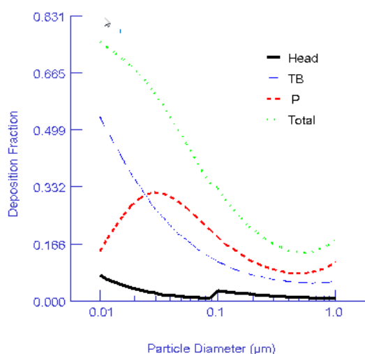
Fig. 8. Predicted deposition fraction for different size particle size using MPPD model.
