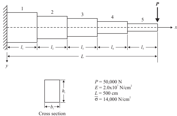
Fig. 1 Cantilevered beam example problem
