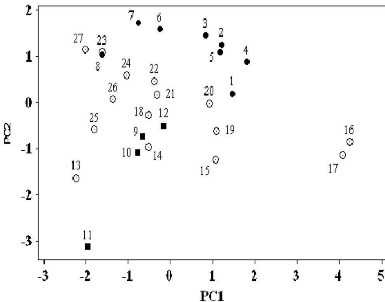
Fig. 1. A plot of the scores of PC2 against PC1 for the systems in Table 6: filled circles represent the biological phases Nos 1– 8, squares represent the biological processes Nos 9 – 12, circles represent the solvents Nos 13 – 27.
