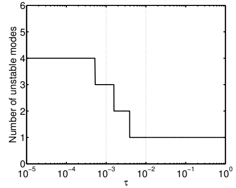
Fig. 19 The number of unstable Fourier modes as a function of the dimensionless time step \tau with N = 100 .
