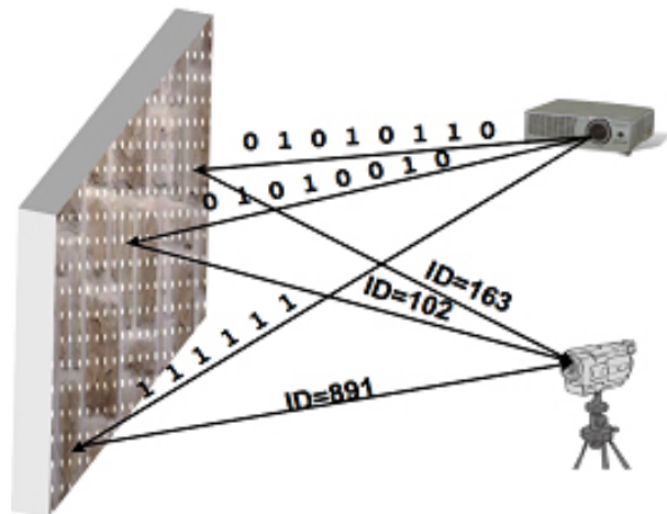
Figure 2: Active registration using binary coded point patterns.
