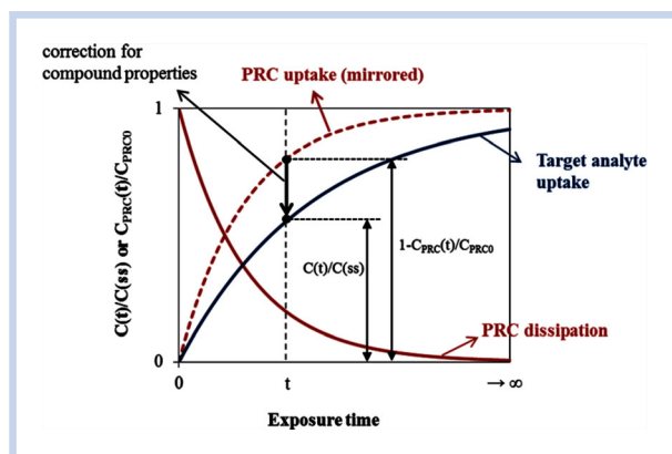
Figure 3. PRC dissipation and compound uptake kinetics generally assumed for the performance reference compound (PRC) approach. C(t) and C(\text{ss}) refer to target analyte concentrations in the passive sampler at time t and steady state, respectively; C_{\text{PRC}}(t) and C_{\text{PRC}(0)} refer to PRC concentrations in the passive sampler at time t and 0, respectively.
