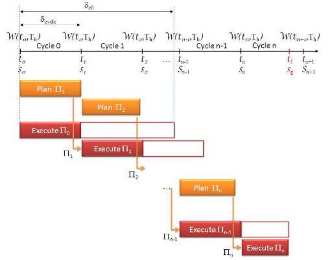
Fig. 2: PASSPMP process.
