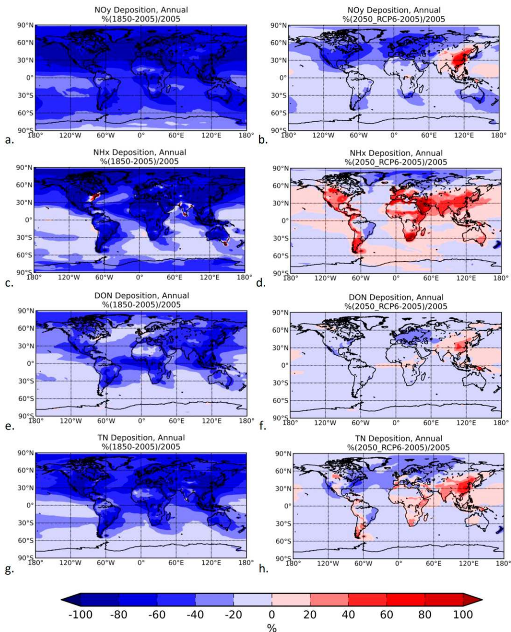
FIG. 4. Percentage change relative to 2005 annual deposition flux computed by TM4-ECPL for (a),(b) NO y ; (c),(d) NH x ; (e),(f) DON; and (g),(h) TN due to (left) preindustrial emissions and (right) anthropogenic RCP6.0 emissions.
