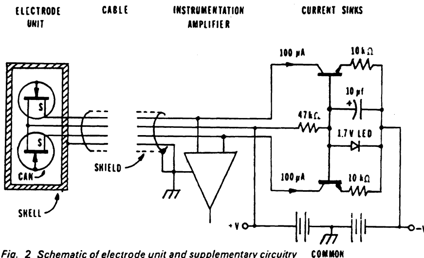
Fig. 2 Schematic of electrode unit and supplementary circuitry
