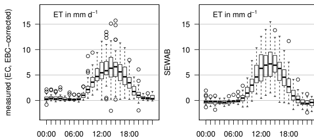
Figure B2. Mean diel course of measured and energy balance corrected evapotranspiration ET (left panel) and SEWAB modelled ET (tile approach according to the EC footprint: S_{RefEC} , right panel) over 61 days during 2010 (3 June to 2 August) at Kema: box plot with median, 25 % and 75 % quartiles; bars represent quartiles \pm 1.5 times interquartile range, dots are outliers. Measured and modelled values are restricted to high flux data quality (flag 1–3). Measured data is corrected according to the surface energy imbalance with the buoyancy flux correction.
