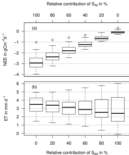
Figure 9. Modelled daily net ecosystem exchange (top, NEE) and modelled daily evapotranspiration (bottom, ET) for 46 days (12 July to 26 August 2012) at Kema (varying combination of S_{\text{IM}} and S_{\text{BS}} ): box plot with median, 25 % and 75 % quartiles; bars represent quartiles \pm 1.5 times interquartile range.
