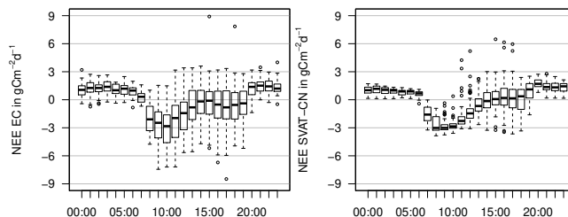
Figure B3. Mean diel course of measured (left panel) and modelled (tile approach according to the EC footprint: S_{RefEC} , right panel) net ecosystem exchange (NEE) over 61 days of 2010 (3 June to 2 August) at Kema: box plot with median, 25 % and 75 % quartiles; bars represent quartiles \pm 1.5 times interquartile range, dots are outliers. Measured and modelled values are restricted to high data quality (flag 1–3 out of a scheme ranging from 1 to 9, Foken et al., 2004).
