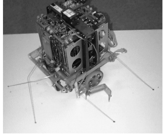
(b) The tactile sensors designed specifically for the Wall-following basic behavior.
