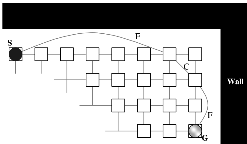
Figure 6 – Exploded view of C-space states showing adjacency (lighter lines). All lighter lines represent spatial adjacency except those labeled F for Follow Wall behavioral adjacency and C for Cornering behavioral adjacency.
