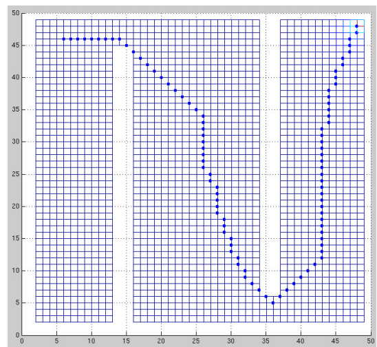
(b) Path computed by optimal potential field method over a 50x50 regular grid (white areas without grid-lines denote obstacle configurations).
