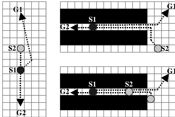
Figure 4 – Solutions to the three most common cases of independently planned intersecting trajectories (clockwise from left): (a) Find non-intersecting trajectories. (b) Vehicle 2 must wait before proceeding into the ‘corridor’. (c) Vehicle 2 must back-out of the ‘corridor’ and allow vehicle 1 to pass before continuing in to its goal.
