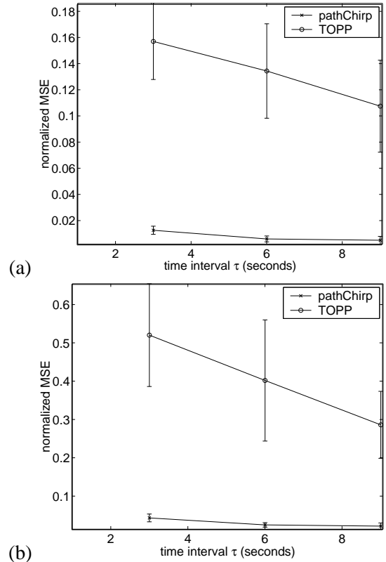
Fig. 11. Comparison of pathChirp and TOPP in a single-hop scenario for two utilizations: (a) 30% and (b) 70%. Observe that pathChirp performs far better than TOPP.
