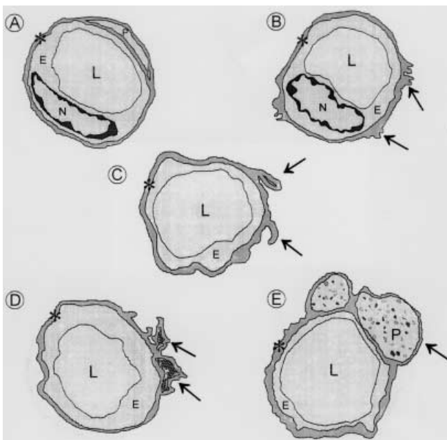
Fig. 1 A–E Schematic drawings representing categories of capillary wall pathology. A A healthy capillary. B Basement membrane thickening pointed at by arrows. C Abnormal duplication and branching of the basement membrane. D Fibrosis. E Pericytic degeneration (L capillary lumen, E endothelial cell, N endothelial nucleus, P pericyte, * basement membrane)
