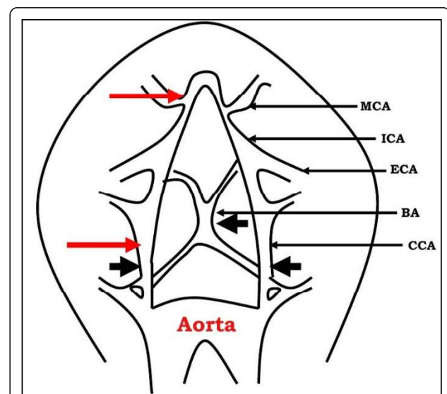
Figure 2 Surgical technique for inducing global or focal cerebral ischemia in mouse. Schematic illustration of arteries demonstrating the three points of occlusion (black arrows) for global ischemia (3-VO) and red arrows for focal ischemia. MCA: middle cerebral artery; ICA: internal carotid artery; ECA: external carotid artery; BA: basilar artery; CCA: common carotid artery.
