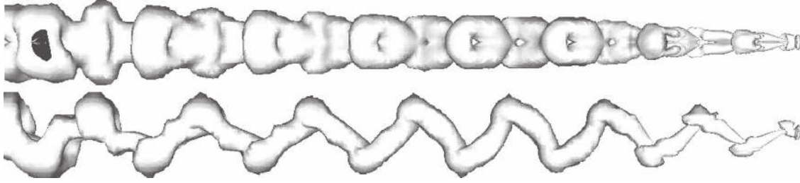
FIG. 8. Two perpendicular views of the wake structure in the zigzagging regime revealed by the \lambda_2 criterion (bubble number 19). The bubble is visible on the right.
