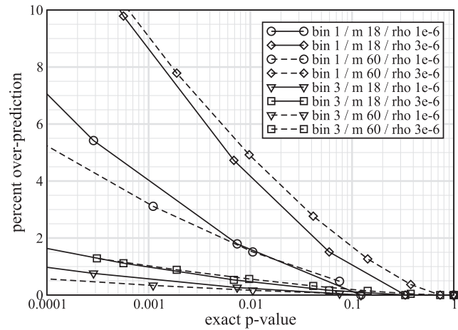
Fig. 2. Percent overprediction of P -values from representative small ( m=18 , solid curves) and large ( m=60 , dashed curves) gene sets. Four scenarios are considered: j=1 bin with background mutation rate of \rho=1/\text{Mb} (circles), j=1 and \rho=3 (diamonds), j=3 and \rho=1 (triangles), and j=3 and \rho=3 (squares). Test sets were generated with randomly selected lengths between 200 and 15000 nt.
