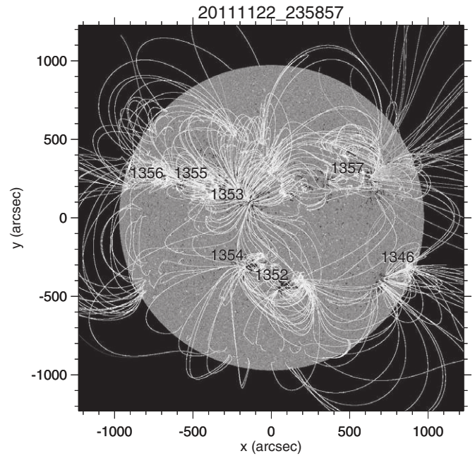
Figure 15. HMI magnetogram, PFSS extrapolation, and AR numbers for case E, 2011 November 22.
