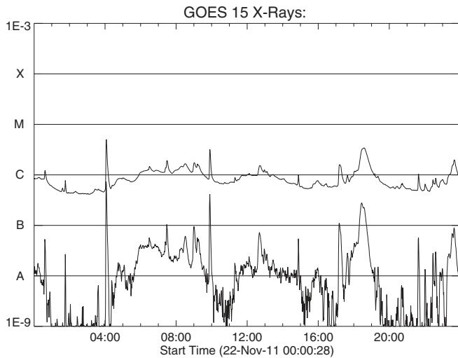
Figure 14. GOES light curve for case E, 2011 November 22.
