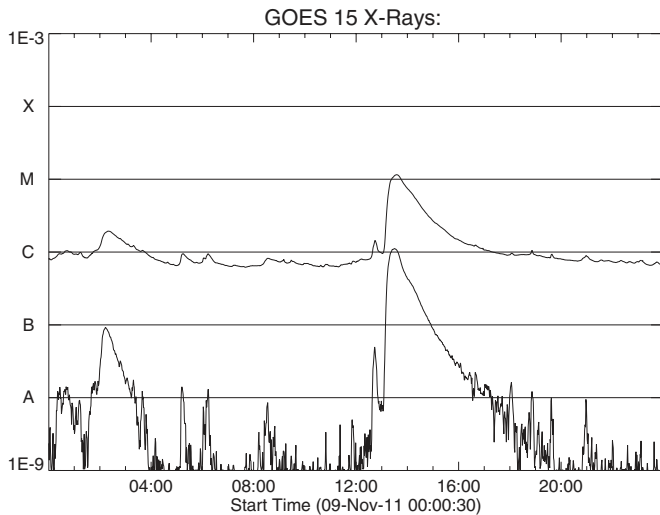
Figure 10. GOES light curve for case D, 2011 November 9.
