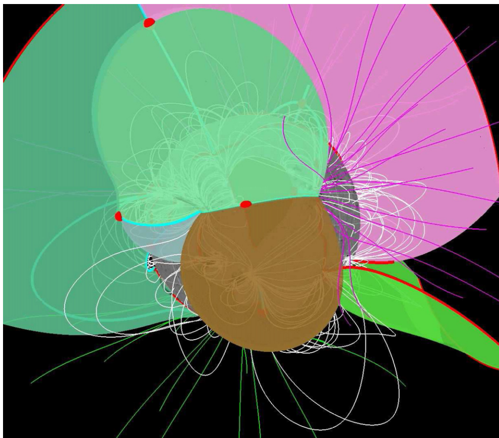
Figure 16. Partial rendering of the topological domains for the PFSS model for case E, 2011 November 22. Selected domain boundaries are shown as translucent surfaces for those separatrices associated with coronal null points (shown as red balls on the blue spine field lines). (A color version of this figure is available in the online journal.)
