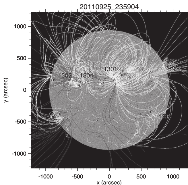
Figure 6. HMI magnetogram, PFSS extrapolation, and AR numbers for case C, 2011 September 25.
