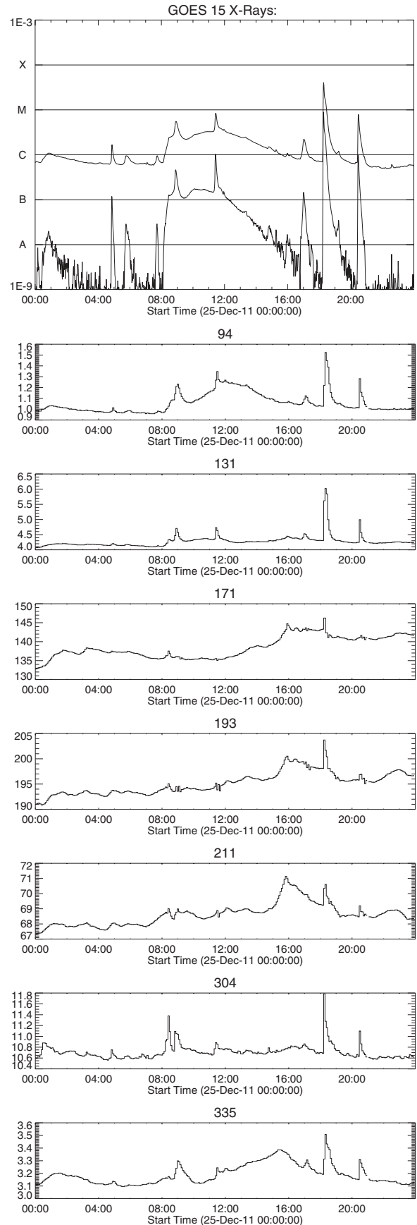
Figure 22. GOES and AIA light curves for case H, 2011 December 25 (for AIA in \text{DN pixel}^{-1} \text{ s}^{-1} ).
