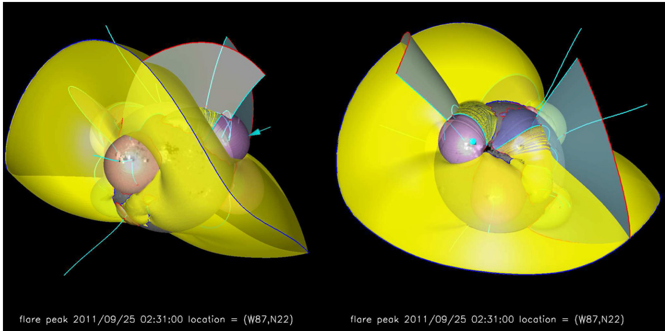
Figure 7. PFSS field topology for case C, 2011 September 25 (cf. Figure 4 for a description of the details). (A color version of this figure is available in the online journal.)
