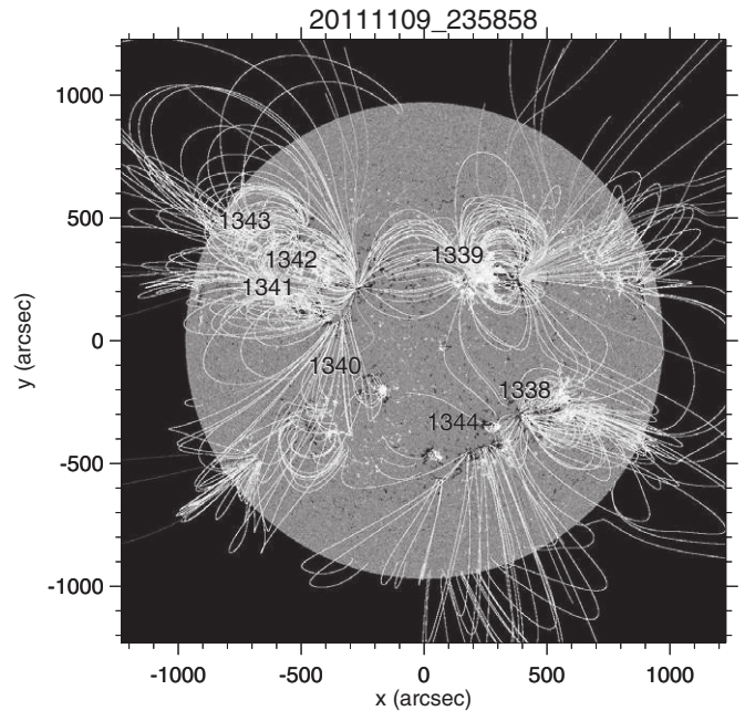
Figure 11. HMI magnetogram, PFSS extrapolation, and AR numbers for case D, 2011 November 9.
