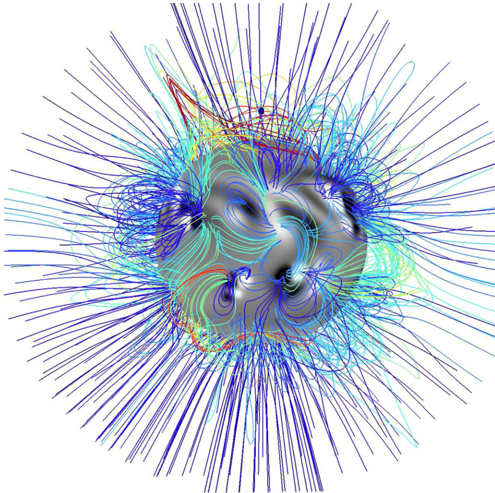
Figure 24. Magnetofrictional field model for case H, 2011 December 25, rotated eastward by 30^\circ relative to the Carrington longitude (cf. Figure 5 for a description of the details).
