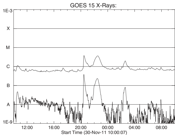
Figure 17. GOES light curve for case F, 2011 November 30.
