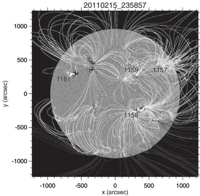
Figure 3. HMI magnetogram, PFSS extrapolation, and AR numbers (showing the last four digits, as is a common standard, here and in subsequent similar figures for other cases) for case B, 2011 February 15.
