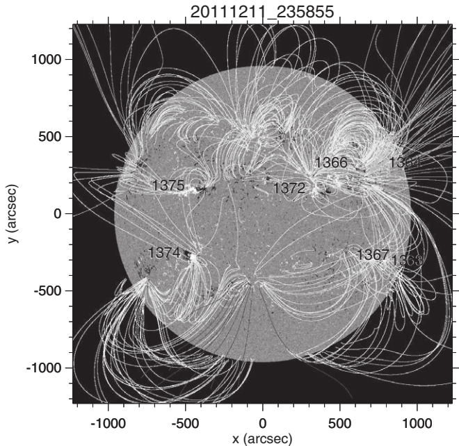
Figure 20. HMI magnetogram, PFSS extrapolation, and AR numbers for case G, 2011 December 11.
