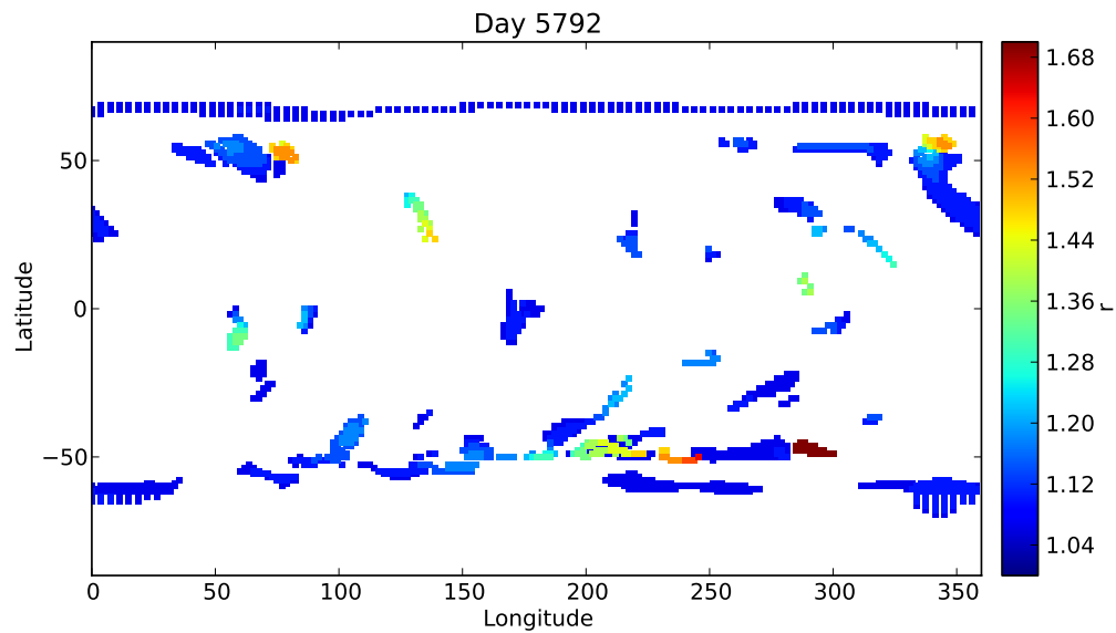
Figure 12. Flux-rope positions, colored by height (see color bar, in units of solar radii), from the magnetofrictional model for case D. The Carrington longitude of disk center on 2011 November 9 is 96^\circ .
