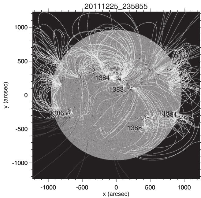
Figure 23. HMI magnetogram, PFSS extrapolation, and AR numbers for case H, 2011 December 25.
