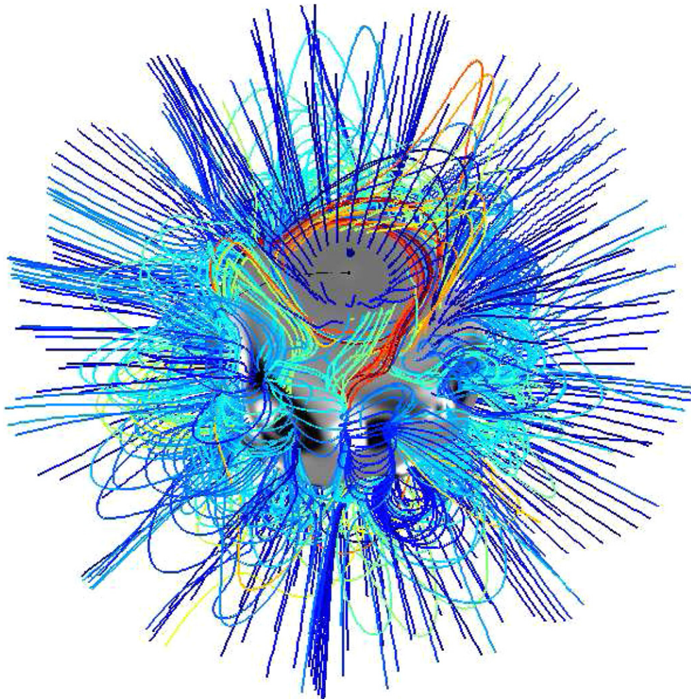
Figure 13. Magnetofrictional field model, tipped to a viewing angle of 57^\circ north latitude for case D, 2011 November 9 (cf. Figure 5 for a description of the details).
