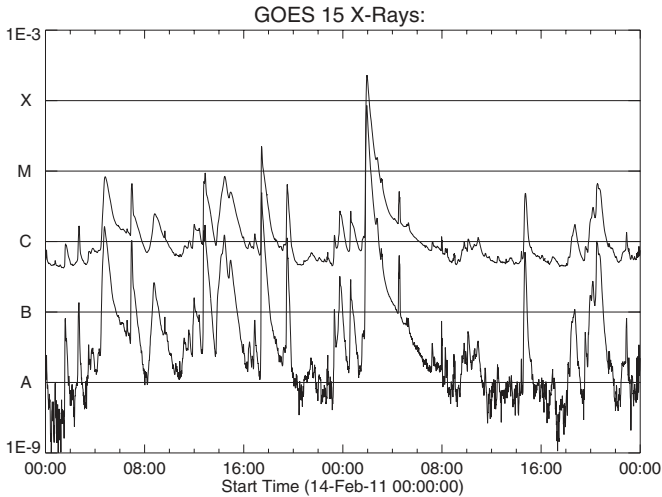
Figure 2. GOES light curve for case B, 2011 February 14–15.
