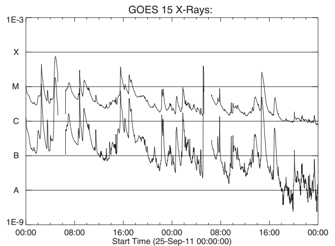
Figure 8. GOES light curve for case C, 2011 September 25.
