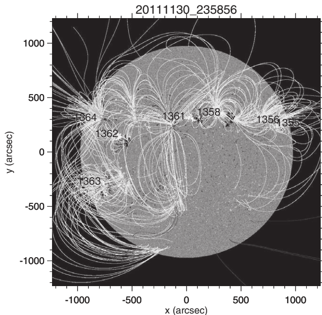
Figure 18. HMI magnetogram, PFSS extrapolation, and AR numbers for case F, 2011 November 30.
