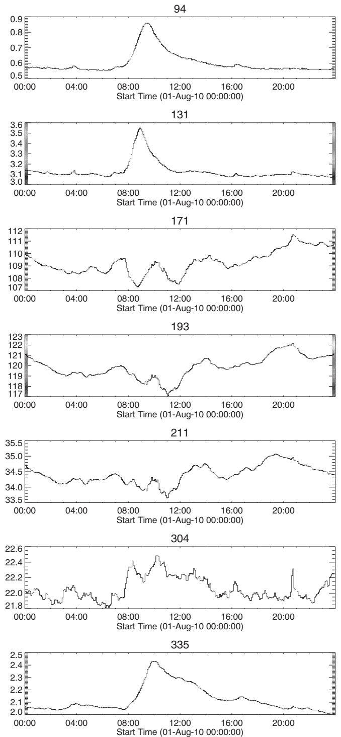
Figure 1. AIA light curves for case A, 2010 August 1 (in DN pixel -1 s -1 ).
