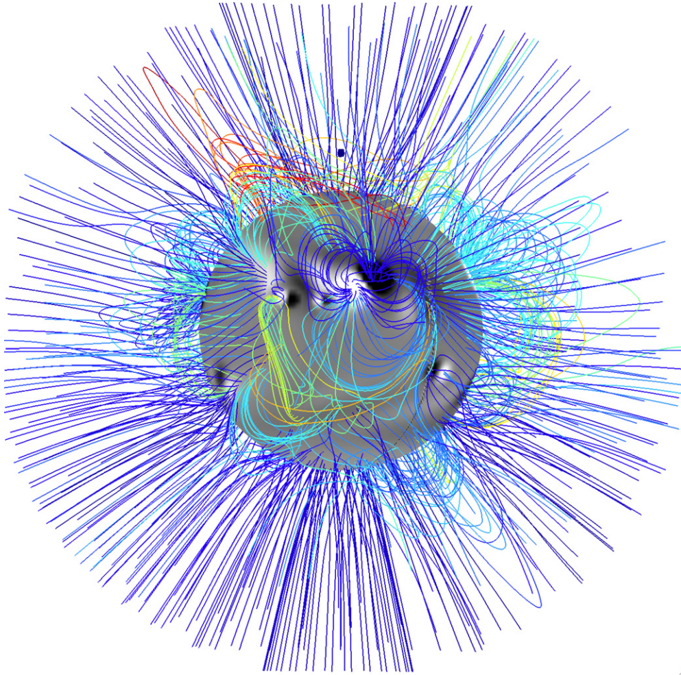
Figure 9. Magnetofrictional field model for case C, 2011 September 25 (cf. Figure 5 for a description of the details). (A color version of this figure is available in the online journal.)
