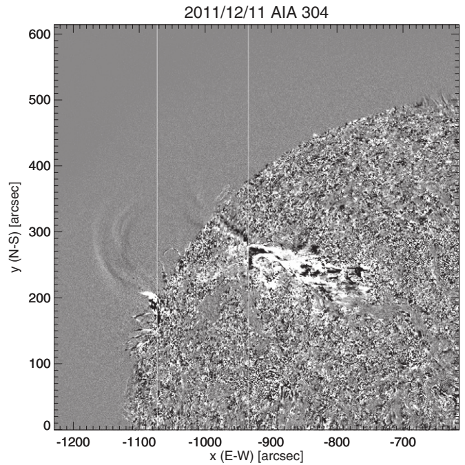
Figure 21. Composite running-difference image for 304 \text{ \AA} exposures on 2011 December 11 (case G), displaying the northeast quadrant of the Sun (summarizing the image sequence shown in the online table 30 that also shows the STEREO images for comparison). This composite image highlights the connection between the on-disk and off-limb erupting regions. The figure is an assemblage of a series of running-difference images, each computed for a time spacing 4 minutes (the image sequence can be accessed online 320 ). To the right of the rightmost vertical white line is the difference image for 05:45 UT, for the early phases of the eruption. To the left of the leftmost vertical line is the image for 07:07 UT. Between the two vertical lines is a series of narrow strips cut out of running-difference images with positions shifting from left to right with time, advancing in steps of 3 minutes, moving in the general direction of motion of the eruption.
