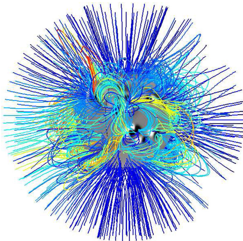
Figure 5. Magnetofrictional field model for case B for 2011 February 16, shown from the Earth perspective on February 14. The field lines are colored depending on the angular spacing of their endpoints in latitude and longitude (regardless of whether they close on the surface or on the source surface) to reduce confusion in closely packed regions and in flux-rope configurations.
