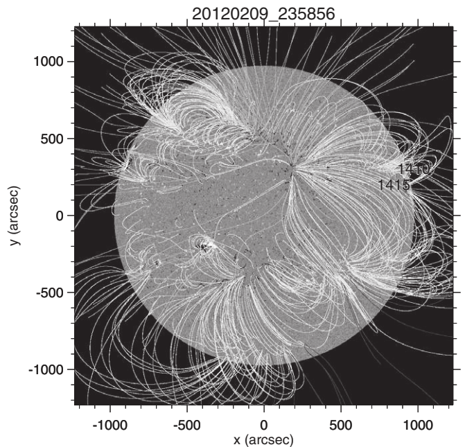
Figure 27. HMI magnetogram, PFSS extrapolation, and AR numbers for case I, 2012 February 9.
