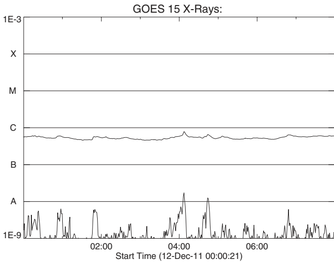
Figure 19. GOES light curve for case G, 2011 December 11.
