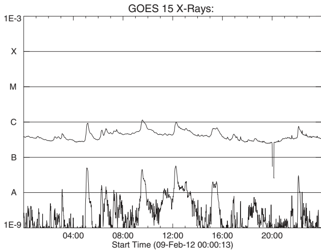
Figure 26. GOES light curve for case I, 2012 February 9.
