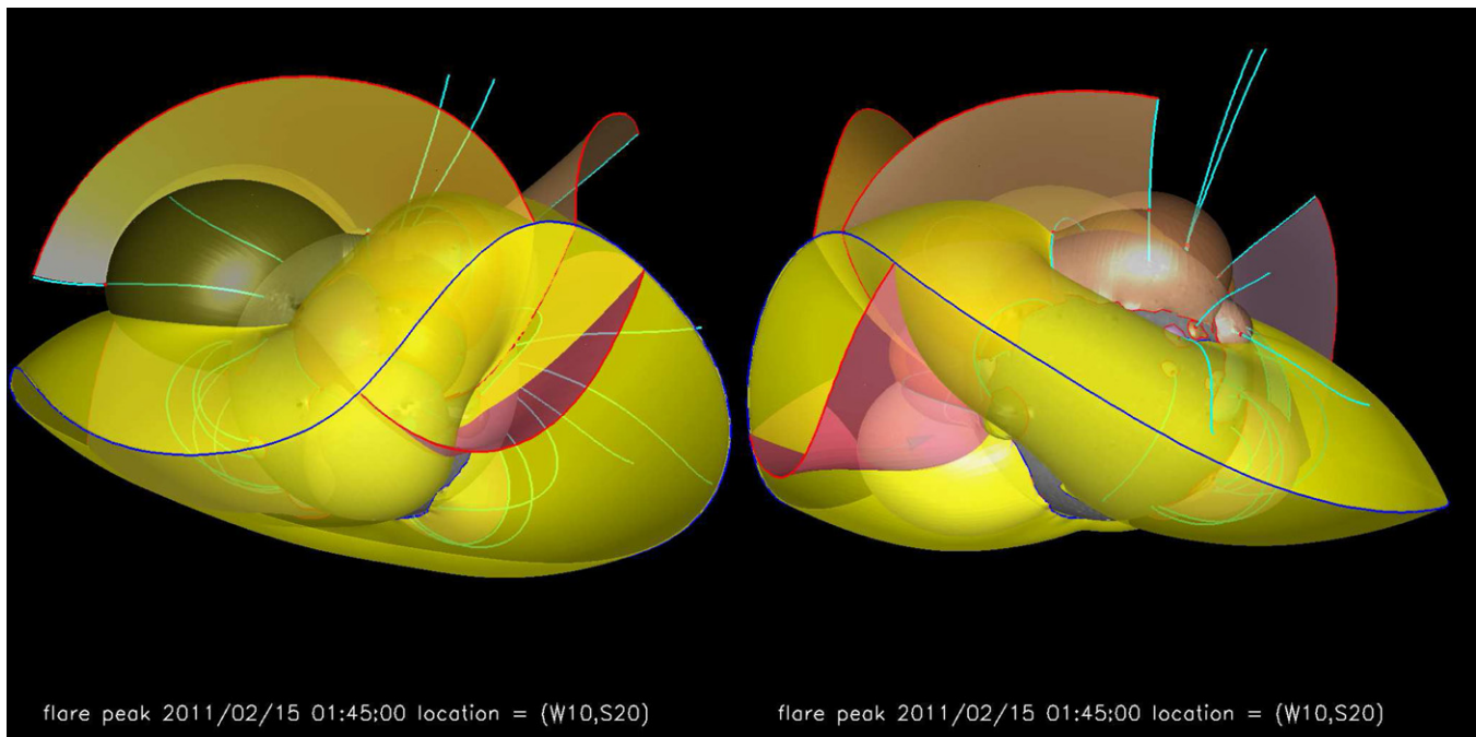
Figure 4. PFSS field topology for case B, 2011 February 15, from the perspectives of Earth and of STEREO-A . The main, yellow, surface is the PFSS helmet, i.e., the envelope of the domain in the solar corona within which all field is closed. At its cusp the radial field component vanishes, so that this cusp forms the basis of the heliospheric current sheet above. Underneath and outside it are other surfaces that are the main topological domains defined by coronal null points (red dots), with their spine field lines shown in light blue. The dark blue curve is the null line for the radial field component on the source surface (at 2.5 solar radii). The red curves are the intersections of the domes and curtains with the solar surface and source surface, respectively. The topological structure shown here and for other cases in this study was computed using the algorithm developed by Haynes & Parnell (2010).
