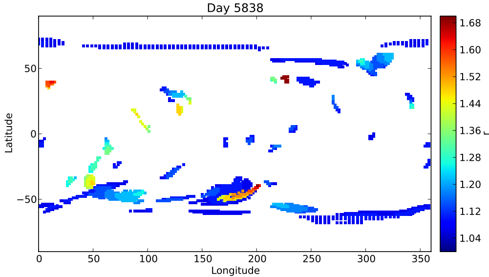
Figure 25. Flux-rope positions, colored by height (see color bar, in units of solar radii), from the magnetofrictional model for case H. The Carrington longitude of disk center on 2011 December 25 is 209°.
