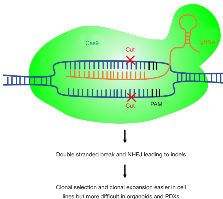
Figure 1 Schematic of CRISPR-Cas9 knockout system. PAM, protospacer adjacent motif; NHEJ, non-homologous end joining; PDX, patient-derived xenograft.
