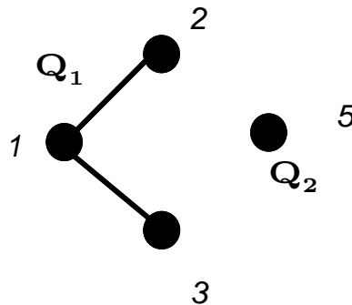
Figure 5. Decomposition of Kite graph KT into KT'
