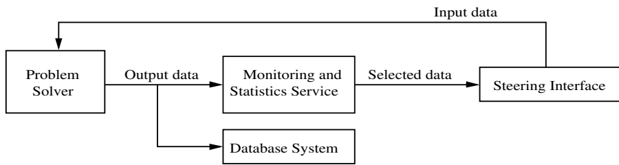
Fig. 3. The initial Monitoring service is replaced with a more complex one (Monitoring and Statistics service), which is activated to continue the filtering of the output data.
