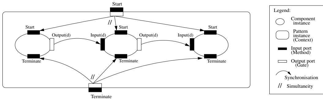
Fig. 16. Example of the Start and Terminate operators over a pipeline pattern instance.
